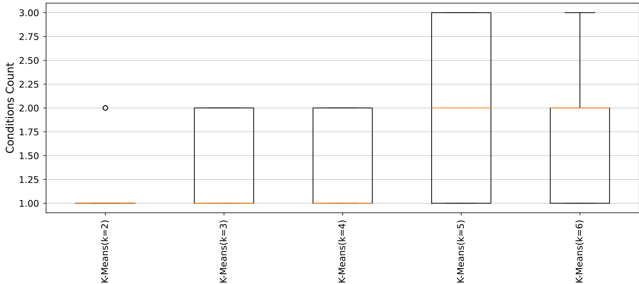
YARA Rules Conditions Count Distribution (Cluster25_Size6 dataset)
